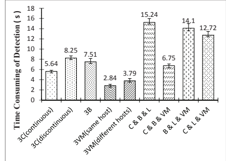
(c) Three nodes failure detection
