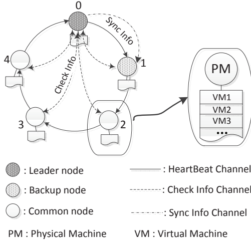
Fig. 2. Smart Ring model
