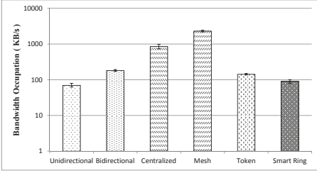
(a) SmartRing VS other models
