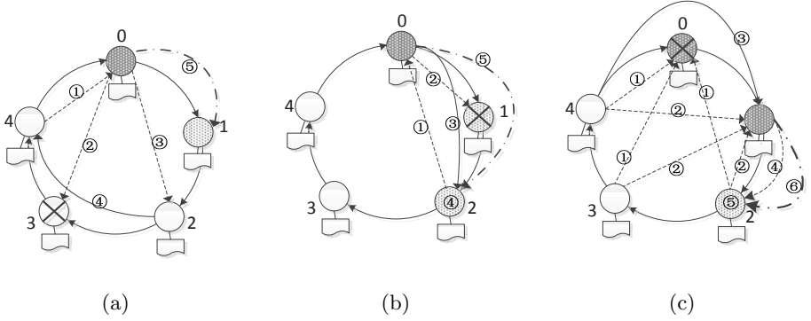
Fig. 3. Node Failure Detection Process. (a)Common node failure detection process. (b)Backup node failure detection process. (c)Leader node failure detection process.
