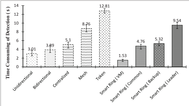
(a) One node failure detection (SmartRing VS other models)
