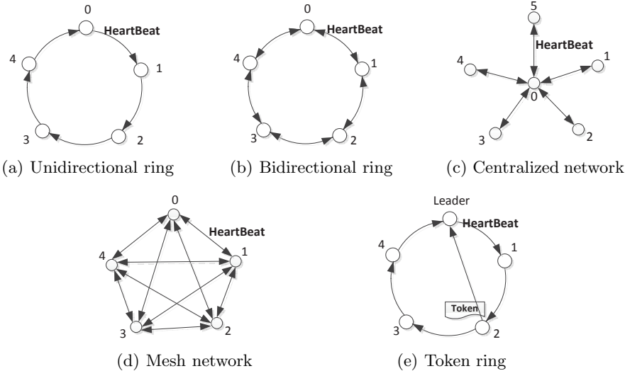
Fig. 1. Traditional node failure detection models
