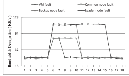
(b) Different node faults in SmartRing
