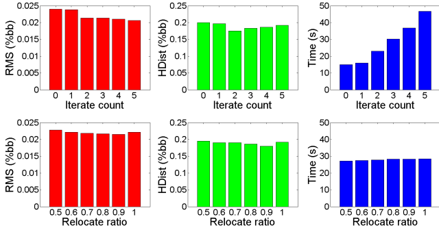
Fig. 15. Effectiveness of the iteration count and relocate ratio. For separability, RMS and Hdlist bars are plotted in different scales. We set \delta = 0.2(\%bb) , and \theta = 30^\circ . The above data are the averages of 10 consecutive executions with the Homer model (Table. 2) as input.
