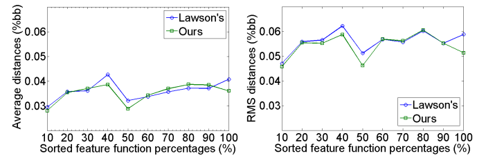
Fig. 14. Comparison of geometric fidelity between Lawson's weighing scheme [44] and ours(Eq. 12). We sort the vertices in M_I according to their saliency function values in ascending order, and compute their average distance and RMS distance in each bin. In this experiment, \delta = 0.2\% (%bb), and \theta = 30^\circ . The above data are the averages of 10 consecutive executions with the Hand model (Fig. 10) as input.
