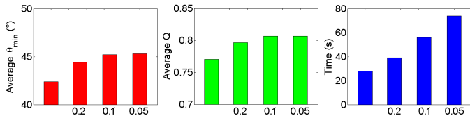
Fig. 17. The effectiveness of \Delta\theta in Alg. 4. In each sub figure, the first bar indicates the value when no final vertex relocation is applied. In this experiment, \delta = 0.2(\%bb) and \theta = 30^\circ . The above data are the averages of 10 consecutive executions with the Helmet model (Table. 2) as input.
