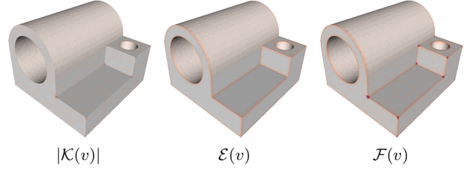
Fig. 8. From left to right Gaussian curvature |\mathcal{K}| , feature edge intensity \mathcal{E} and combined feature intensity \mathcal{F} , with higher intensities in red.
