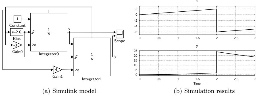
Figure 1: A miscompiled Simulink model (R2009b) ♣
