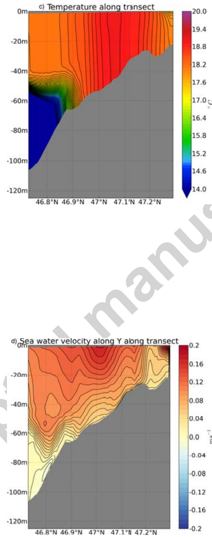
Figure 12: Remotely sensed sea surface temperature (a), modeled sea surface temperature (b), temperature (c) and meridional velocity (d) along transect (black line on (b)) from the PREVIMER model simulations on 26/10/2006.
