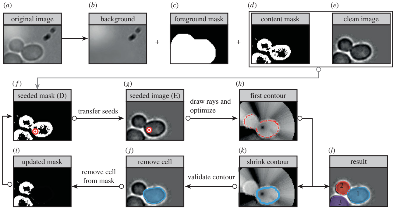
Figure 2. Segmentation pipeline: preprocessing, seeding and contour deformation. The background ( b ) is computed and subtracted from the original image ( a ) to give the clean image ( e ). Preprocessing steps also include the computation of the foreground ( c ), cell border (not shown) and cell content ( d ) masks. These masks are used to place initial seeds, represented by red/white dots ( g ). Starting from each seed, the initial shape of the snake ( h ) is computed by drawing concentric rays, computing an approximated E_{\text{snake}} and selecting its minimum along each ray; the initial shape of the snake is modified according to the given regularity constraints to obtain the final contour ( k ). After filtering (figure 3), selected contours ( j ) are removed from the border and content masks, as shown in ( i ) so as to ease the discovery of new cells. The final result is shown in ( l ).
