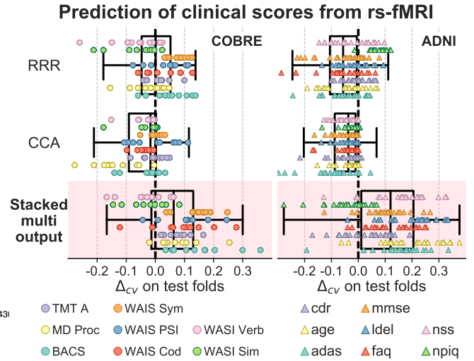
Figure 7: Comparing multi-output stacking to Canonical Correlation Analysis CCA and Reduced Ranked Regression (RRR) on COBRE and ADNI. Stacked multi-output models predict better than other multi-output analysis methods. Results are consistent across datasets.
