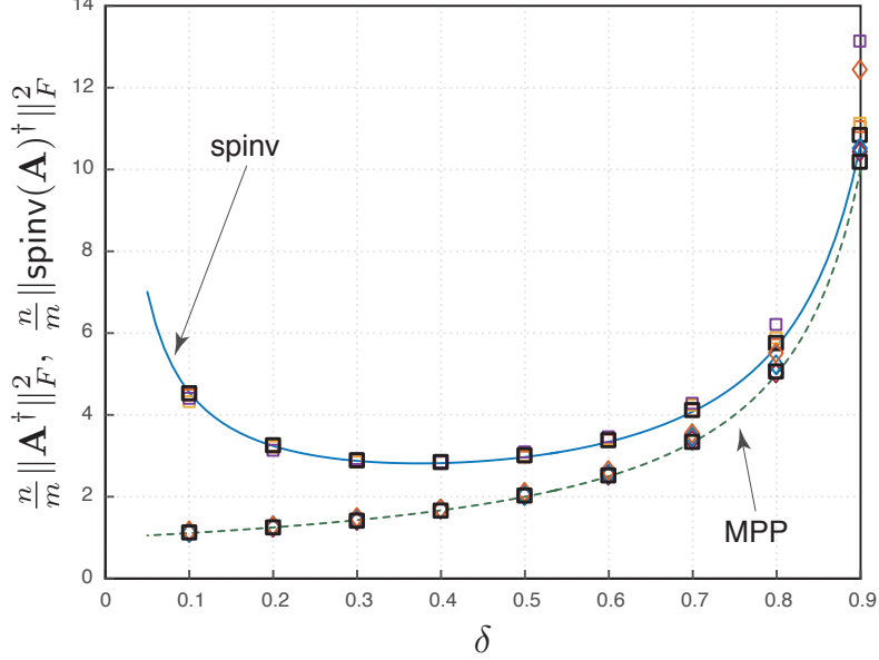
Figure 3: Comparison of the limiting (\alpha_p^*)^2 with the mean of \frac{n}{m} \|\mathbf{A}^\dagger\|_F^2 and \frac{n}{m} \|\text{spinv}(\mathbf{A})^\dagger\|_F^2 for 10 realizations of \mathbf{A} . Empirical results are given for \delta \in \{0.1, 0.2, \dots, 0.9\} and n \in \{100, 200, 500, 1000\} . Black squares represent the empirical result for n = 1000 ; colored squares represent the empirical mean of \frac{n}{m} \|\mathbf{A}^\dagger\|_F^2 for n \in \{100, 200, 500\} , with the largest discrepancy (purple squares) for n = 100 ; colored diamonds represent the empirical mean of \frac{n}{m} \|\text{spinv}(\mathbf{A})^\dagger\|_F^2 with the largest discrepancy (orange diamonds) again for n = 100 .
