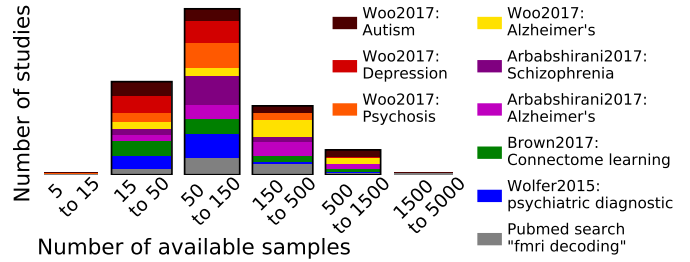
Figure 2: Sample sizes in neuroimaging studies A stacked histogram compounding sample sizes from multiple sources: the Woo et al. (2017) review paper, differentiating Autism, Depression, Pyschosis, and Alzheimer’s studies, the Arbabshirani et al. (2017) review paper, differentiating Schizophrenia and Alzheimer’s studies, the Brown and Hamarneh (2016) review on prediction from connectomes, and the Wolfers et al. (2015) review on prediction for psychiatric disorders, as well as the 100 first answers to a pubmed search on “fmri decoding”. The total histogram comprises 642 studies, with a median number of samples of 89.
