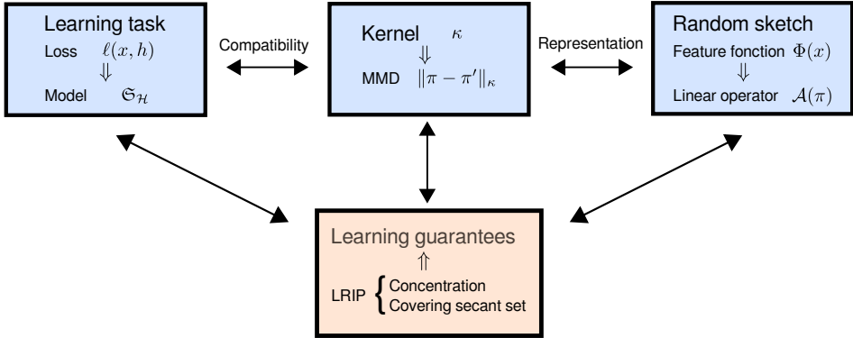
Figure 1: A representation of the links between different concepts in this paper.
