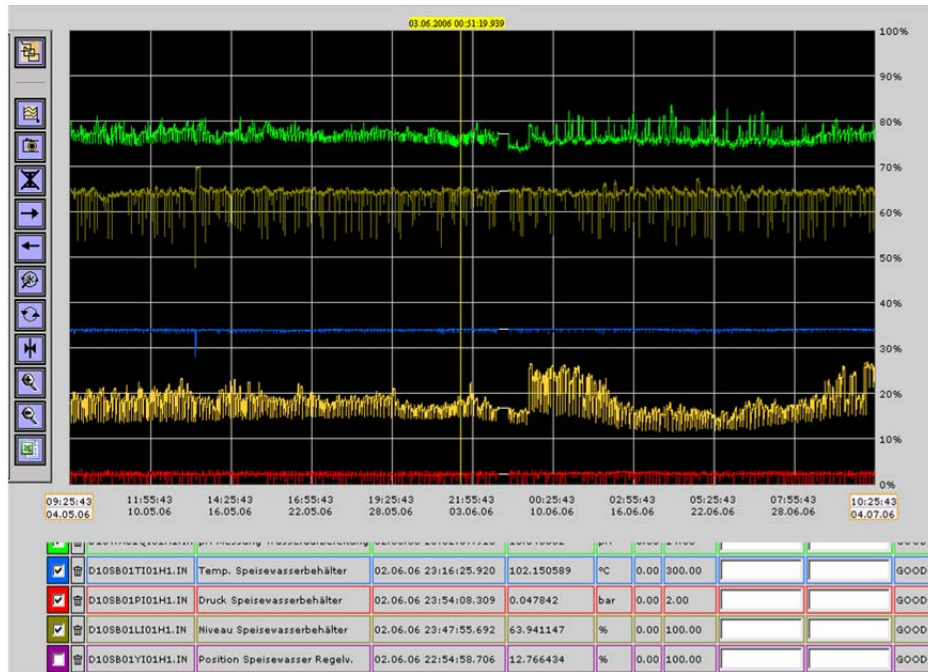
Figure 1. The user interface of the decision support system, called AutoDyn
