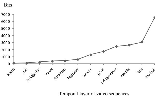
Fig. 7. The relation between motion feature of video sequence and bits at temporal scalability.
