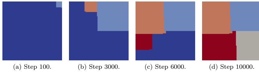
FIGURE 8: Steps of KGGGP while partitioning a 100 \times 100 grid graph in 4 parts. The free part is colored in blue. This part becomes empty at the final step (10000) showing a 4-way partition.
