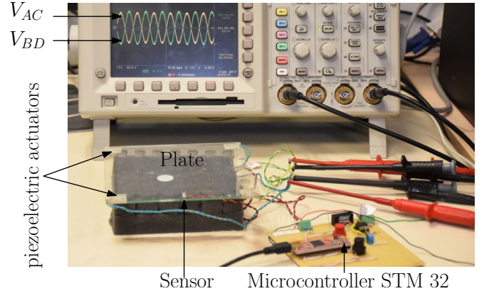
Fig. 6. Experimental setup
