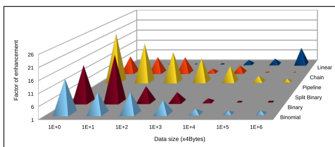
Figure 7: Enhancement factor of hierarchical approach for Open MPI Broadcast implementations SMP12E5 (96 cores)
