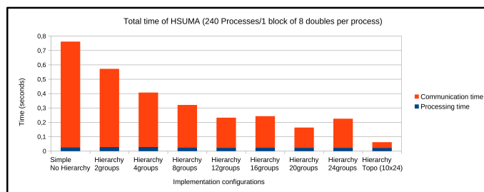
Figure 11: Comparison of execution time of simple, topology-oblivious hierarchical and topological matrix multiplication implementations on NTW10E5. 240 processes process 1 block of 8 doubles
