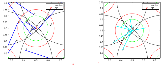
(a) Stable matching resulting from Gaussian cost and BDAA. (b) Matching resulting from the best-RSSI scheme.
