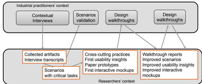
Fig. 2. Our case study research methodology
