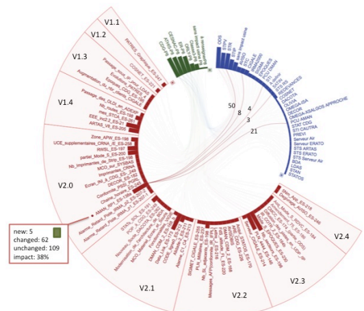
Fig. 7. a chord diagram visualization for release planning
