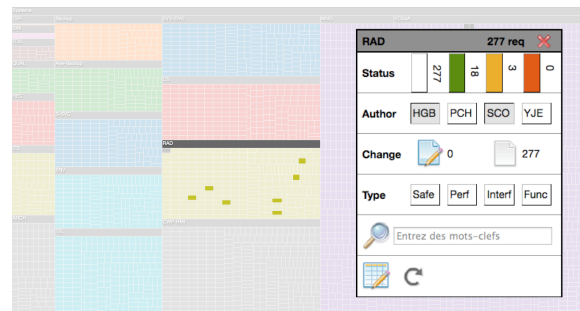
Fig. 6. A requirement inspector for interactive filtering
