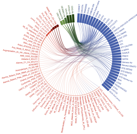
Fig. 7. a chord diagram visualization for release planning
