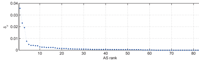
Fig. 3. Worst affected ASes with HARNET
