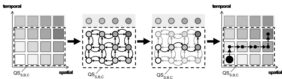
Fig. 2: The steps of interpreting the SVC layer model as graph, retrieving the path with minimal variation from it, and interpretation as adaptation path
