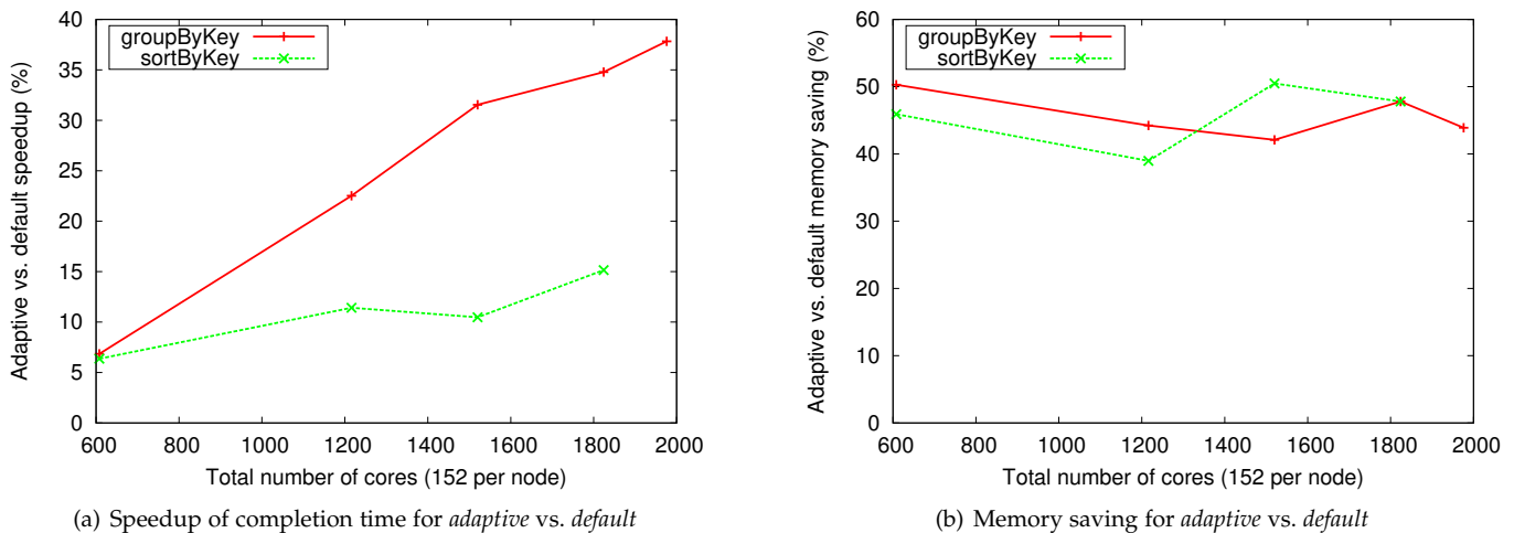
Fig. 4. Weak performance scalability and memory efficiency for an increasing number of nodes and problem scale using a reducer in-flight limit of 10 MB. Higher is better.
