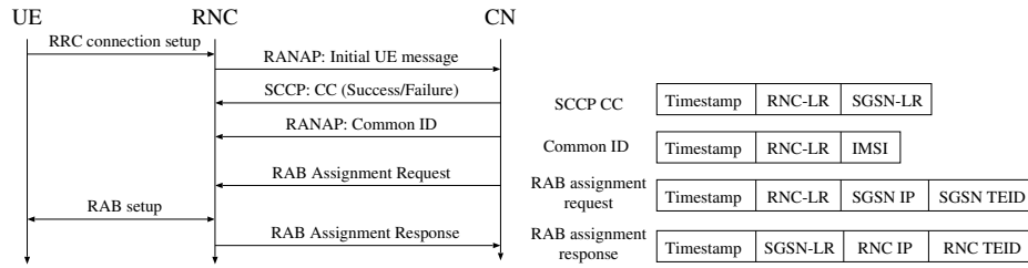
Fig. 2. Signaling message flow of the RRC connection setup.
