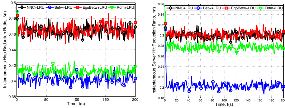
Fig. 3. Instantaneous behavior of the caching schemes for a binary tree: (left) \beta , (right) \gamma .
