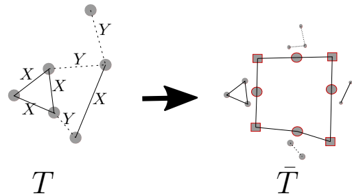
Fig. 1. Example of the construction of \bar{T} . On the righthand side, the round nodes represent connected components of T and the square nodes represent shared vertices.
