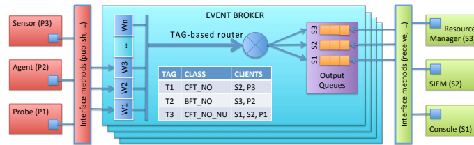
Fig. 2. Broker internal components and event message flow
