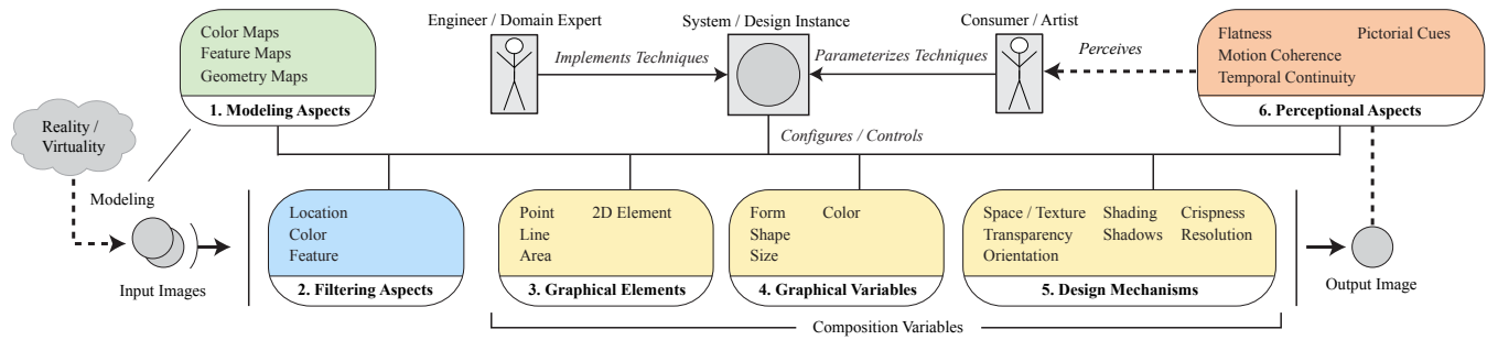
Figure 4: Semiotic structure comprising graphical core variables and mechanisms that may be considered for style transfers.
