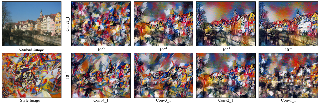
Figure 5: Adjusting the level of abstraction: (top) using different relative weightings between content/style reconstruction, (bottom) matching the style representation with layer subsets of the VGG-Network. Images from Gatys et al. (2016b), © IEEE, used with permission. Style image by Wassily Kandinsky is in the public domain (source: Google Art Project).
