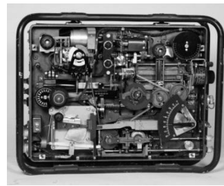
Figure 5: Bombsight computer
