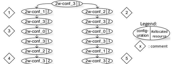
Figure 6: Reconfiguration Tree from the Excerpt of Pairwise Reconfigurations Graph
