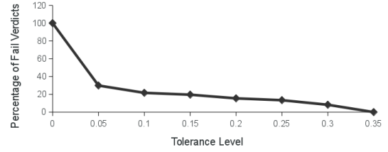
Figure 7: Percentage of Fail Verdicts by Tolerance
