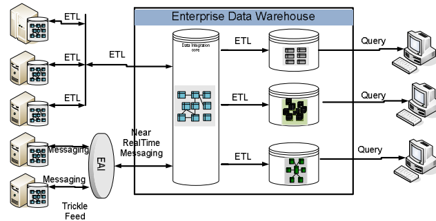
Fig. 1. Coexistence implementation style with trickle feed
