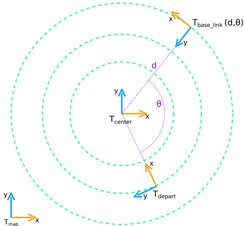
Figure 3.3: Coordinate Frames for a single robot used by the navigation algorithm: The robot's dynamic position T_{base\_link} is defined with respect to three static reference points. The reference of the SLAM algorithm T_{map} , the center point of the scene T_{center} , and the point of depart of the robot T_{depart} marking the zero of the angle \theta that defines the displacement on a circle.
