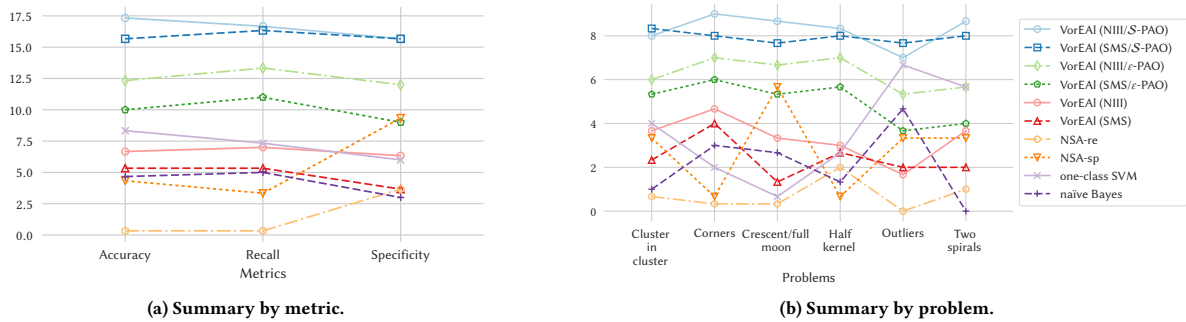
Figure 4: Summaries of the statistical tests by problem and metric. Higher values are better.
