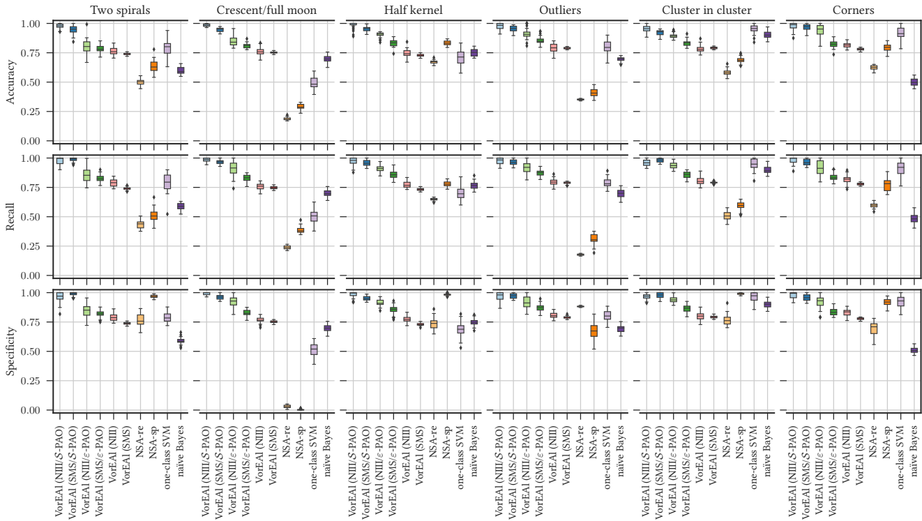
Figure 3: Box plots of the different combinations of S -PAO and \epsilon -PAO heuristics and selection operators based on NSGA-III (NIII) and SMS-EMOA (SMS), VorEAI without using the PAO heuristics and the other methods included in the comparison.
