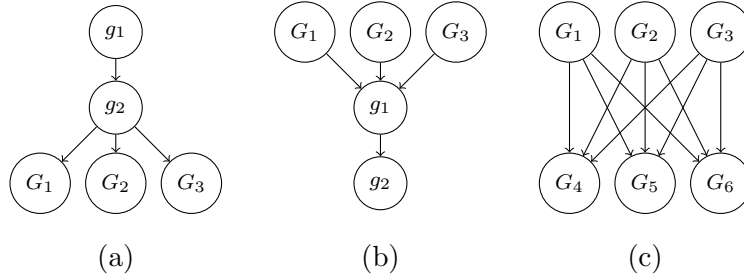
Figure 1: Example M-SPG structures: (a) fork: (g_1 \vec{\rightarrow} g_2) \vec{\rightarrow} (G_1 || G_2 || G_3) ; (b) join: (G_1 || G_2 || G_3) \vec{\rightarrow} (g_1 \vec{\rightarrow} g_2) ; (c) bipartite: (G_1 || G_2 || G_3) \vec{\rightarrow} (G_4 || G_5 || G_6) .
