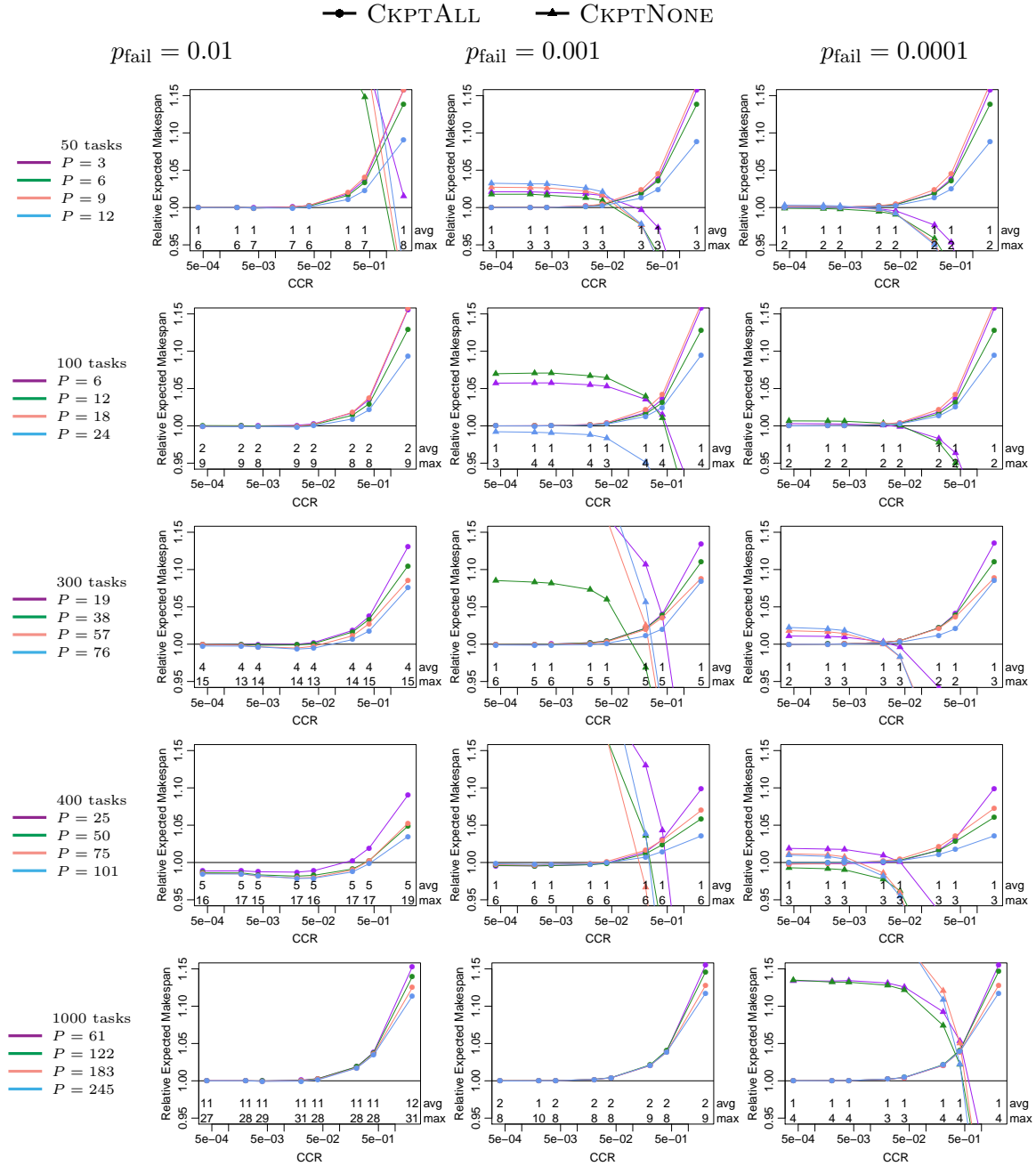
Figure 10: Expected makespan of CKPTALL and CKPTNONE relative to that of CKPT-SOME for the LIGO workflow, three different failure rates, five workflow sizes, and varying Communication-to-Computation Ratio (CCR).
