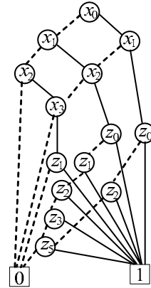
Fig. 4. ZBDDs for translation function
