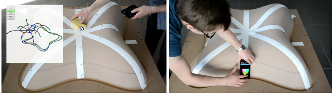
Figure 11: The devices used for data acquisition. Left: the Morpherider and a screenshot of the MATLAB acquisition interface. Right: a standard smartphone and the application with a simple acquisition interface.
