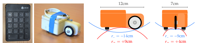
Figure 10: Left: the Morphorider and the wireless keypad that we use for marking nodes during acquisition. Right: the schema shows Morphorider's limitations with respect to radius of curvature at locally convex (red) and concave (blue) surface points.
