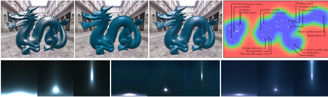
Figure 3: Real-time exploration of our BRDF manifold. 3 materials (red points) are chosen manually, in the vicinity of blue-acrylic , by clicking in the 2D latent space (top right). The latent variables were optimised using all 101 materials of the MERL database. Our proposed construction of the BRDF manifold lends itself to real-time rendering (25 fps) using interpolated materials along with all combinations of dynamic geometry, view points and lighting (see sec. 3.3) using zonal harmonics up to L = 40 [Soler et al. 2015]. The slices of the interpolated BRDFs are also visualised. Please see the accompanying video for a live demonstration.
