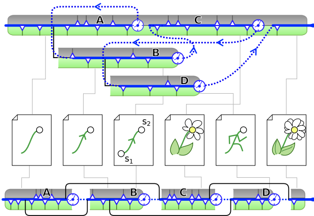
Figure 1. CAUSALITY overview: branching chronology (top 3 rows); linear timeline (bottom, and blue line in top 3 rows); lettered and illustrated states match in both visualizations. Application context is the grey bar; Artifact state is the green bar. Commands shown as blue triangles; time-travel as clocks and dotted lines within the linear timeline. Black strokes between states represent branching in both visualizations.
