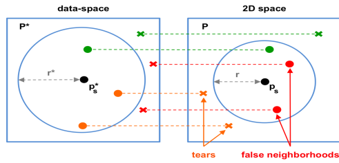
Figure 2: Model characterizing the different types of points relative to the reference point (in black). The neighborhood of the reference in the data-space is represented by a sphere of radius r^* centered in the reference p_s^* . And in the same way, its neighborhood in the 2D space is represented by a disc of radius r centered in p_s . Points in the neighborhood of the reference are represented by a circle and the other by a cross. The points are either topological artifacts, i. e. false neighborhoods (in red) and tears (in orange), or well placed points (in green).
