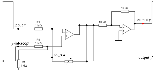
Fig. 1. Hardware model of a straight-line generator based on Op-Amp-technique. Transfer characteristic of a two-stage amplifier represents a straight line in PP.
