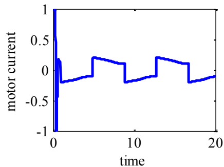
Fig. 8. Motor current.
