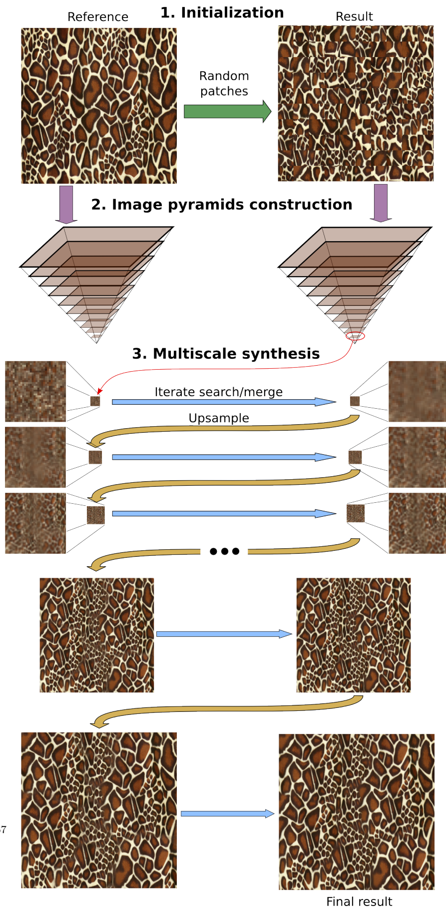
Figure 10: Texture synthesis algorithm. See text for details.
