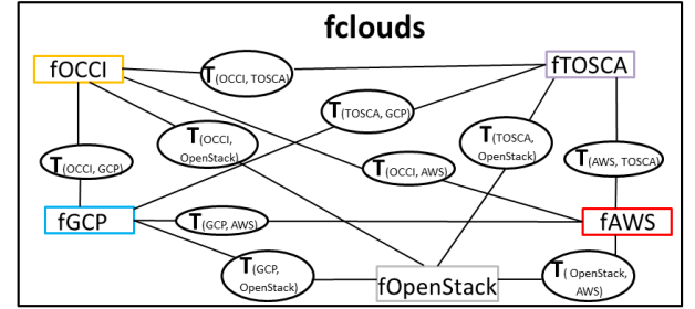
Fig. 3: FLOUDS Framework Overview.
