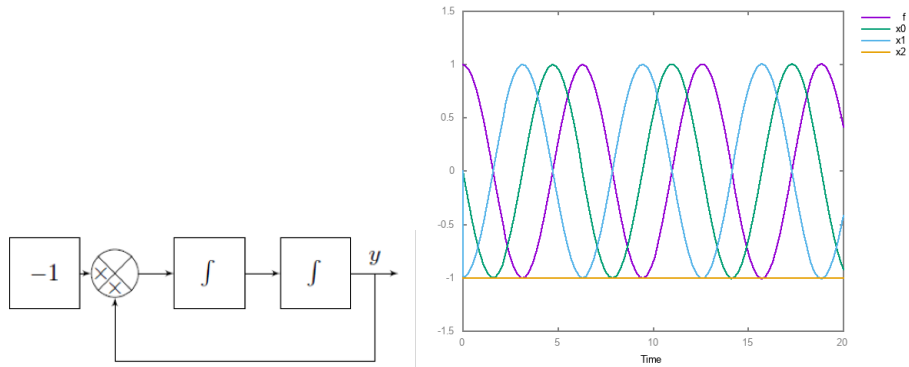
Fig. 1. GPAC circuit for generating the cosine function as a function of time, and numerical simulation trace.
