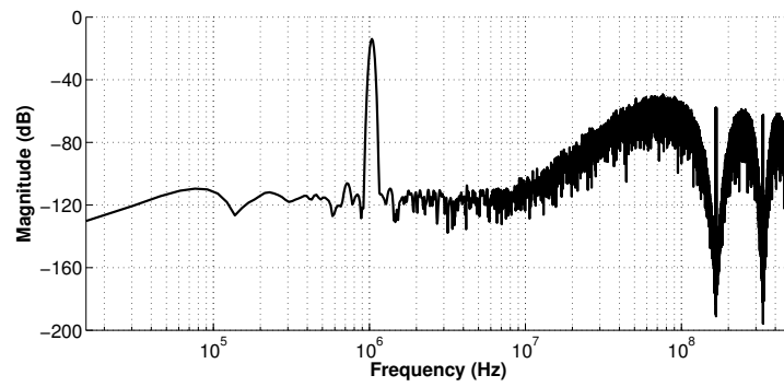
Fig. 8. Output spectra for: (a) p = 3 , (b) p = 4 , (c) p = 5 , (d) p = 6 .
