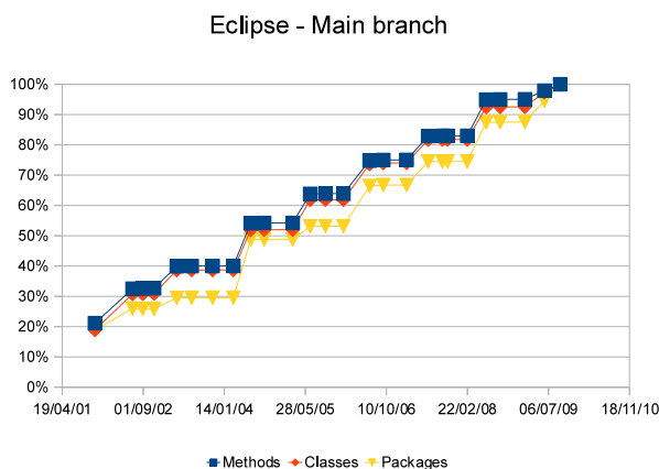
Fig. 2. Growth in the “main” branch of Eclipse
