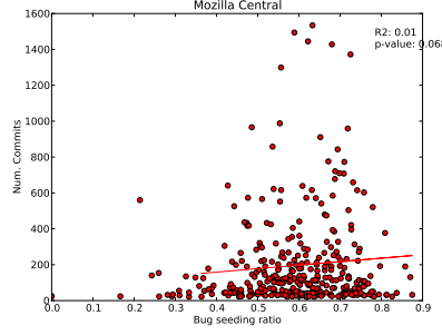
Fig. 1. Correlation study between number of commits and the bug seeding ratio. Each dot represents a developer of the Mozilla Central repository (Firefox project).
