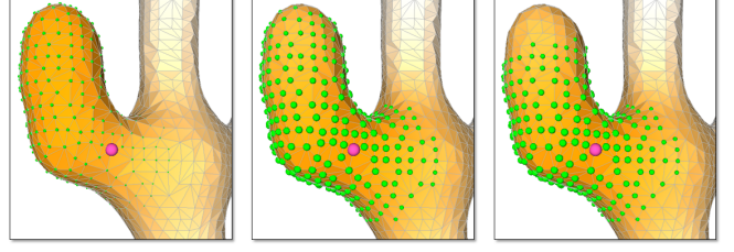
Fig. 4. Choice of weighting functions. From left to right: K_t(x, x_i) , K_t(x, x_i)/\sqrt{K_t(x, x)K_t(x_i, x_i)} and 2K_t(x, x_i)/(K_t(x, x) + K_t(x_i, x_i)) for x indicated as the purple vertex. Its neighborhood, i.e., vertices x_i for which W_x(x_i) > \varepsilon , is shown with green spheres proportional to function values.
