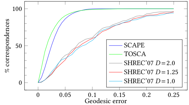
Fig. 18. Evaluation on benchmark datasets. We plot the percentage of correct correspondences against geodesic error, averaged over all model pairs, for various datasets. Our curves for SHREC’07 show three different bounds on allowed mass distortion.
