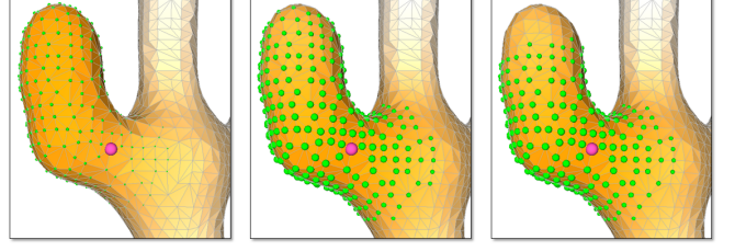
Fig. 4. Choice of weighting functions. From left to right: K_t(x, x_i) , K_t(x, x_i) / \sqrt{K_t(x, x) K_t(x_i, x_i)} and 2K_t(x, x_i) / (K_t(x, x) + K_t(x_i, x_i)) for x indicated as the purple vertex. Its neighborhood, i.e., vertices x_i for which W_x(x_i) > \varepsilon , is shown with green spheres proportional to function values.
