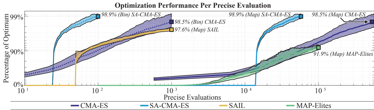
Figure 7. Optimization Efficiency in a Single Bin and Over the Entire Design Space Computational efficiency of CMA-ES, SA-CMA-ES, MAP-Elites, and SAIL measured in in precise evaluations. Bin : median progress towards optimum in every bin. Map : performance of CMA-ES and SA-CMA-ES is median bin performance multiplied by number of valid bins. Performance of individuals produced to construct initial models is set to 0%. Bounds indicate one standard deviation over 20 replicates. PEs and performance in log scale.
