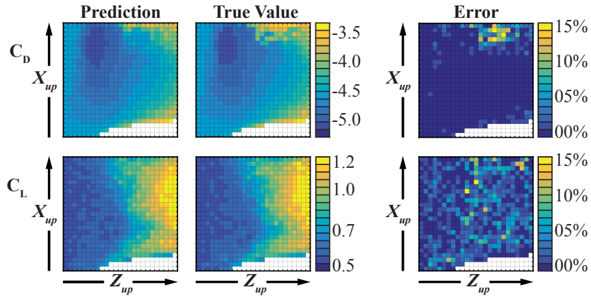
Figure 4. Drag and Lift Predictions and True Value in Each Bin. Predicted and true values of drag and lift for designs in each bin after 1000PE. Median values over 20 replicates.
