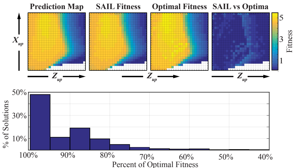
Figure 6. Performance of Designs Found By SAIL Top: Median predicted and true performance of designs found by SAIL with a budget of 1000PE compared with performance of optimal designs found by 20 runs of CMA-ES per bin ( \approx 11.5 million PE) Bottom: Optimality of SAIL designs per bin.
