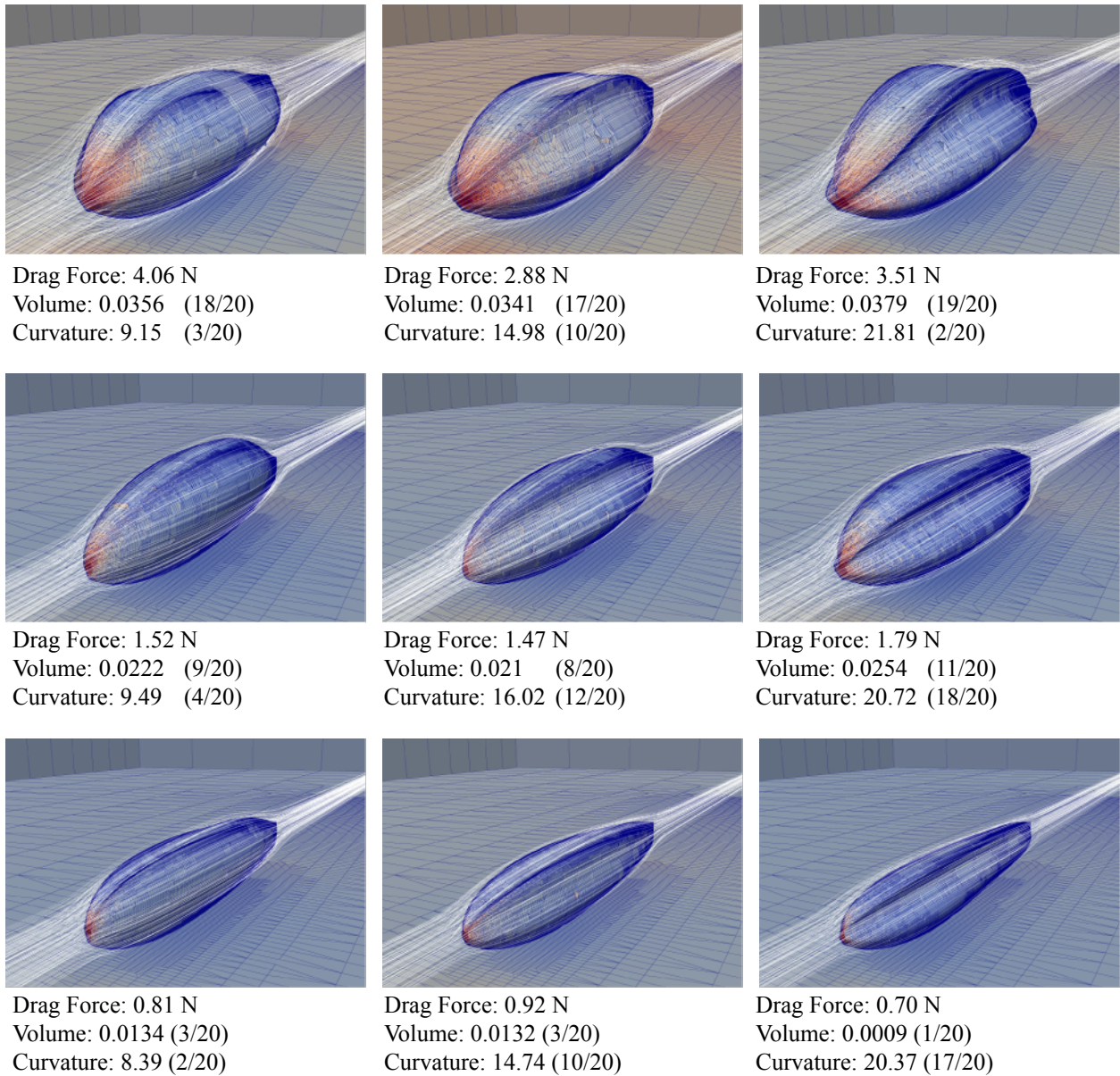
Figure 11. A selection of designs produced in a single run of SAIL. Left: Lower Curvature, Up: Increased Volume Parenthesis after category indicate the bin where each design is located
