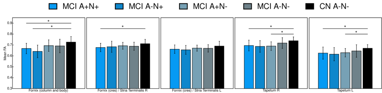
Figure 1. Mean FA in anatomical white matter tracks. Mean FA values for the fornix and the tapetum for which significant differences were found. The bar graph shows mean values (and standard deviation) for each group. * p < 0.05 for Mann Whitney U test. L, Left; R, Right. Abbreviations: FA, fractional anisotropy; L, left; MCI, mild cognitive impairment; R, right.
