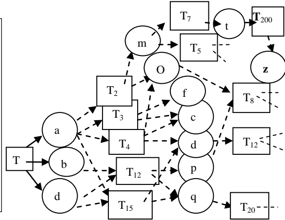
Figure 4. Predictive Dependency Graph Model
